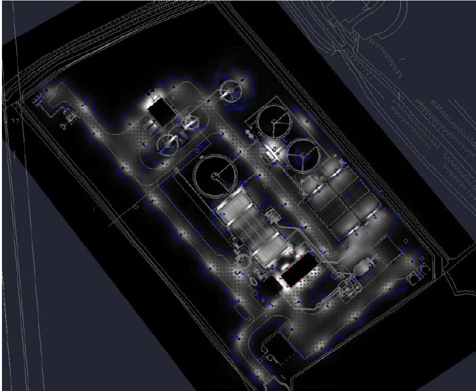
Figure 11-16 : Proposed Lighting Layout Plan
